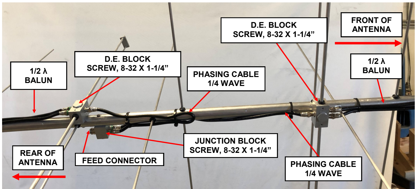
FIG. 3 CABLE ROUTING DIAGRAM WITHOUT POLARITY SWITCH
