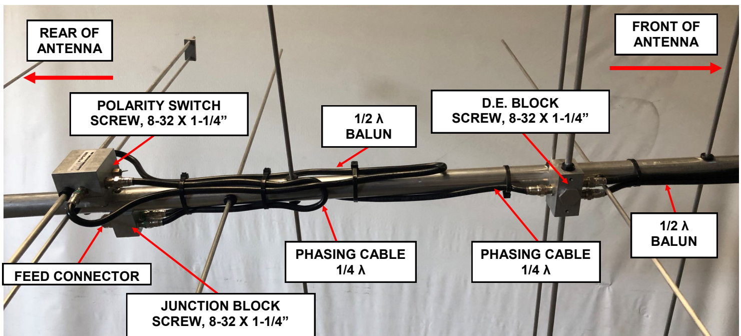
FIG. 4 CABLE ROUTING DIAGRAM WITH POLARITY SWITCH
